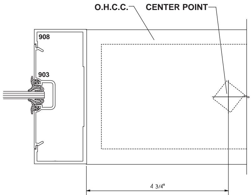
OVERHEAD VIEW
