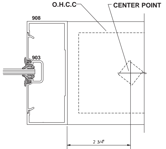
OVERHEAD VIEW
